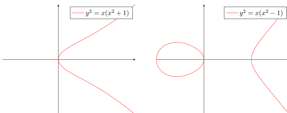
Figure 1.6: the smooth cubics: the second curve demonstrates that the notion of connectedness in the Zariski topology of \mathbb{R}^2 is very different from the one in the usual topology of \mathbb{R}^2 .
