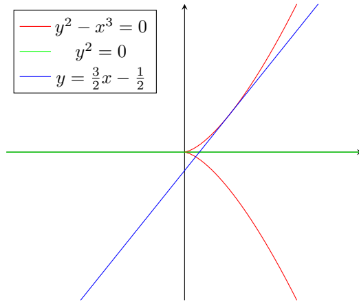
Figure 1.7: The green line is the tangent cone at (0, 0) and the blue line the tangent cone at (1, 1) .
