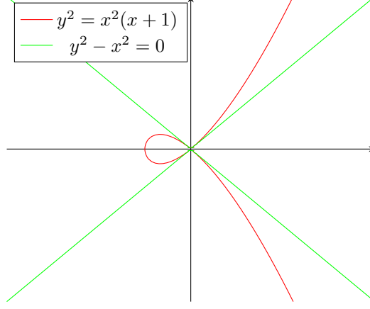
Figure 1.8: The green line is the tangent cone at (0, 0) .
