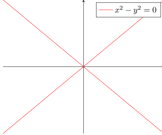
Figure 1.3: Reducible connected algebraic set
